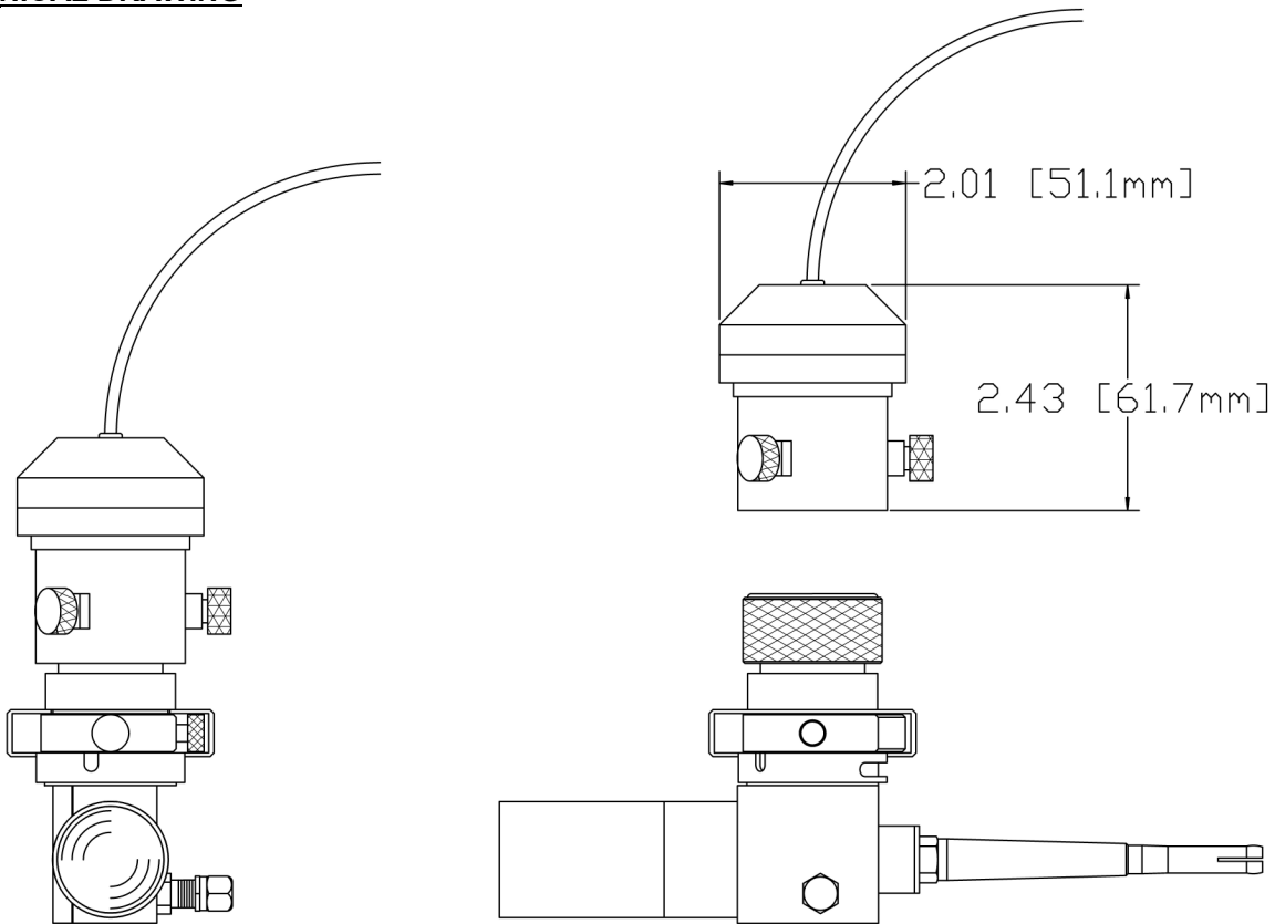
FRONT VIEW (BCA on Boresight)
